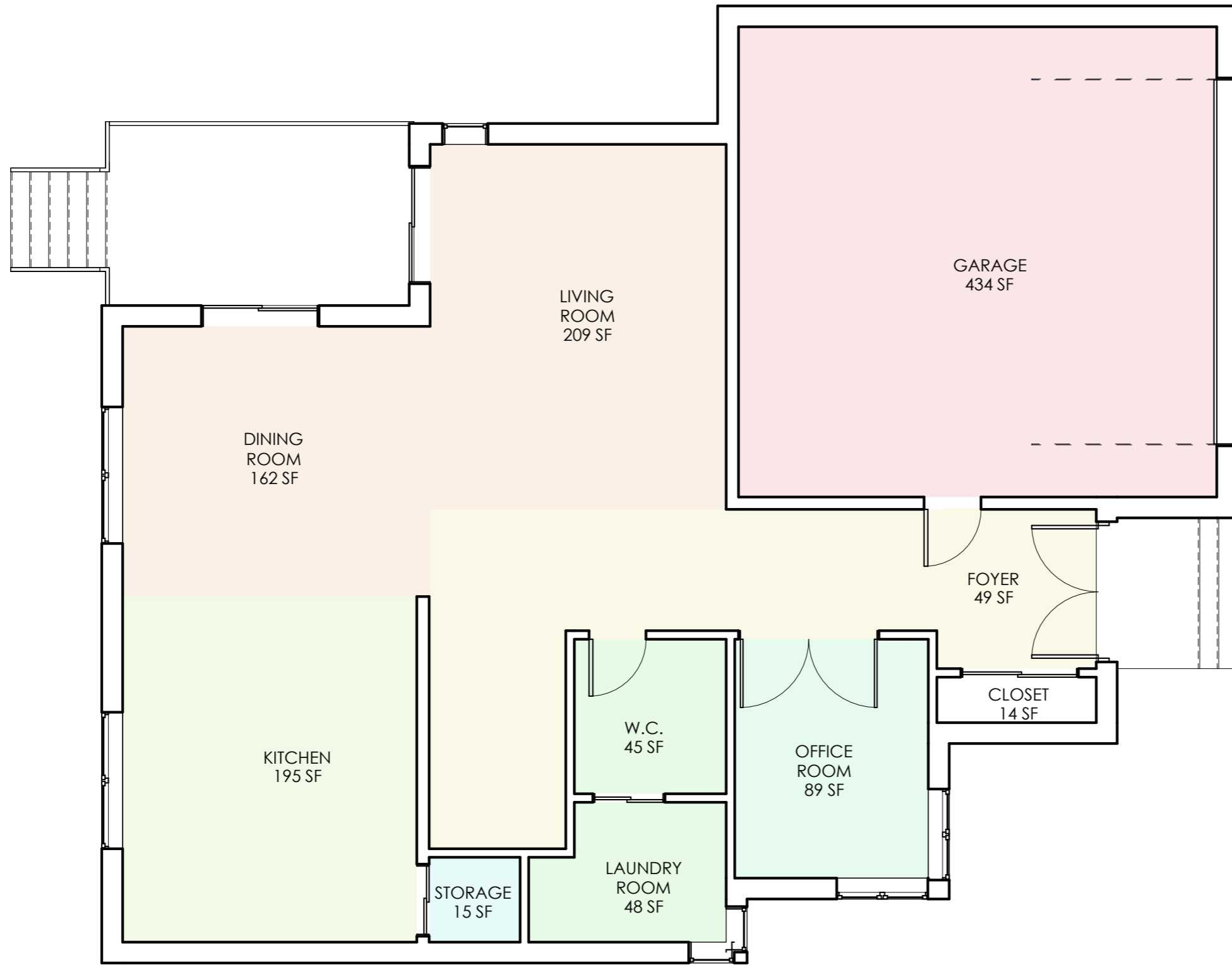
EXISTING GROUND FLOOR PLAN 3/16" = 1'-0"
