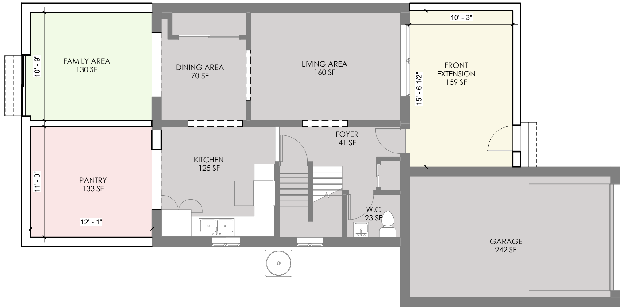
PROPOSED SKETCH 3/16" = 1'-0"
